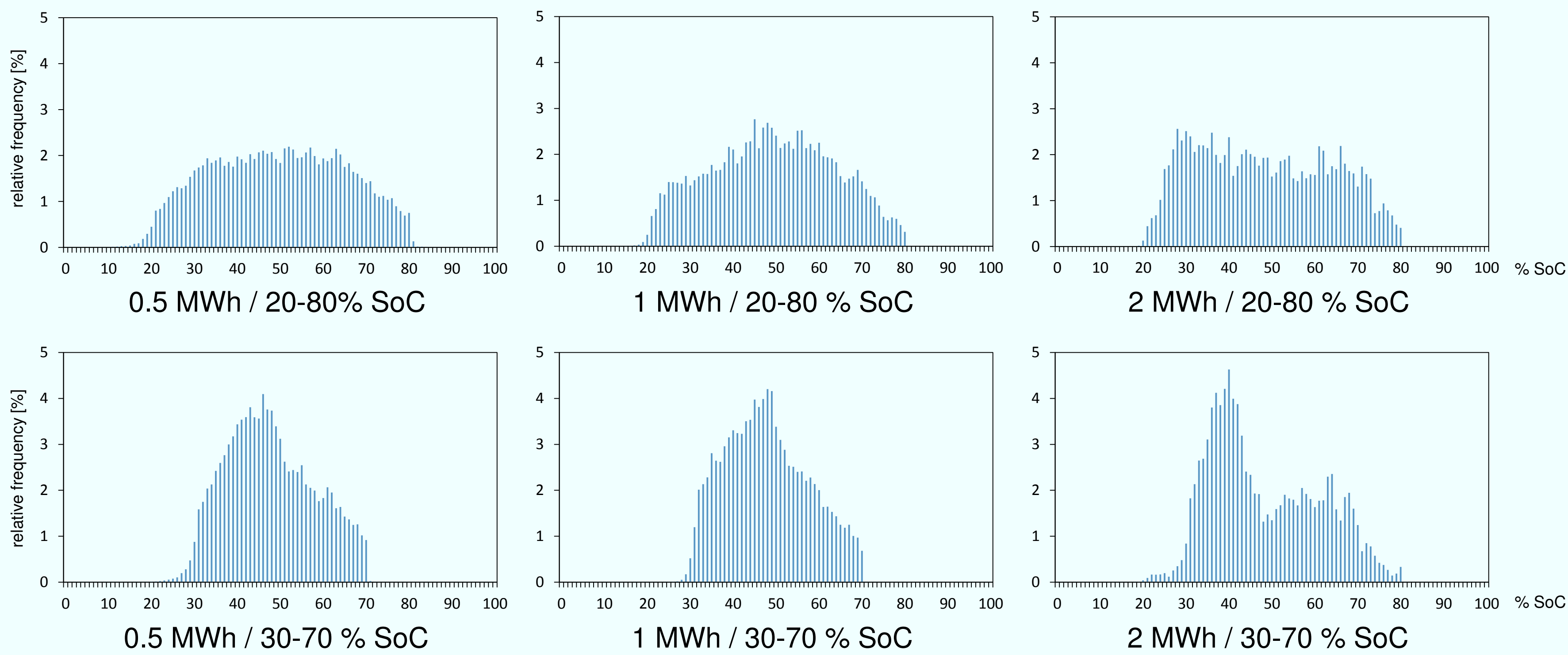
Fig. 6: SoC distributions
