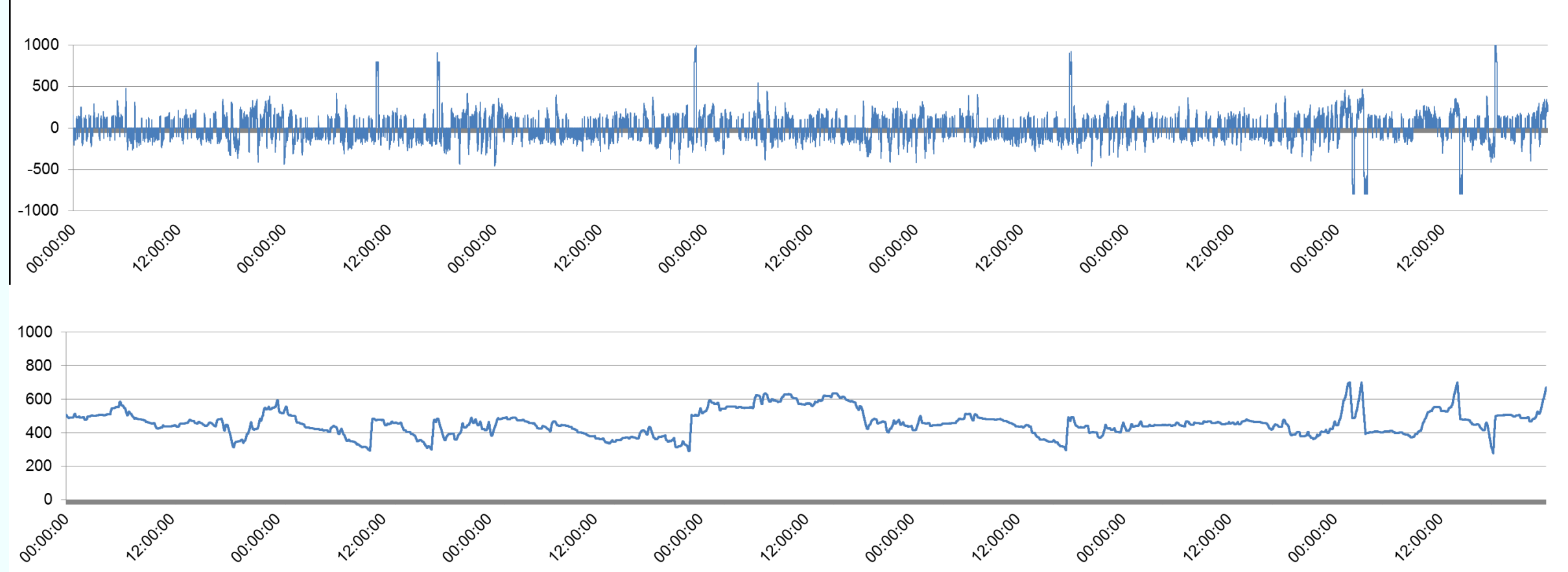
Fig. 2: Exemplary load profile and SoC profile of a battery system providing PCR (1 MW/1 MWh capacity, 30-70% SoC, 1 week operation)
